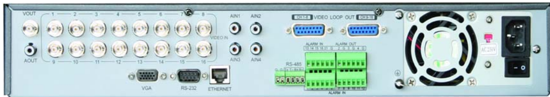
Rear Panel of 16Channel Unit
